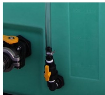
SIGHT GAUGE KIT
